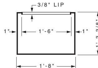
SECTION THRU CONSTRUCTED TANK
