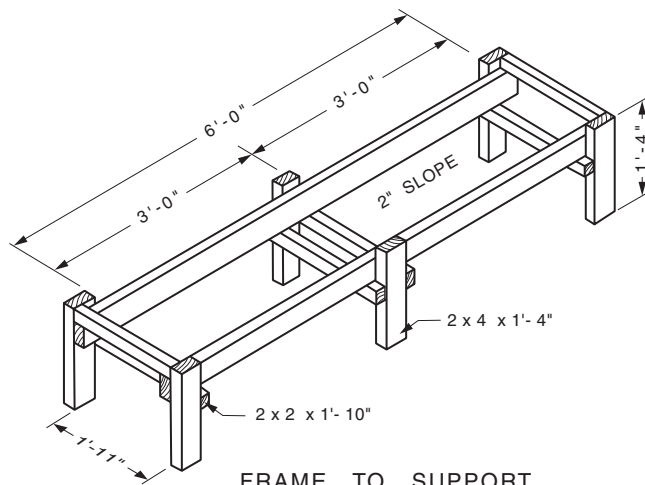
FRAME TO SUPPORT UNCAPPING TANK
