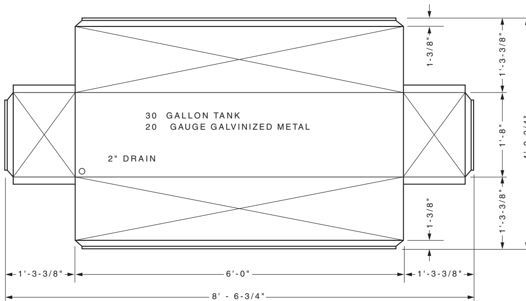
HONEY UNCAPPING TANK
