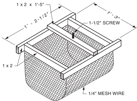
BASKET TO COLLECT WAX CAPPINGS
